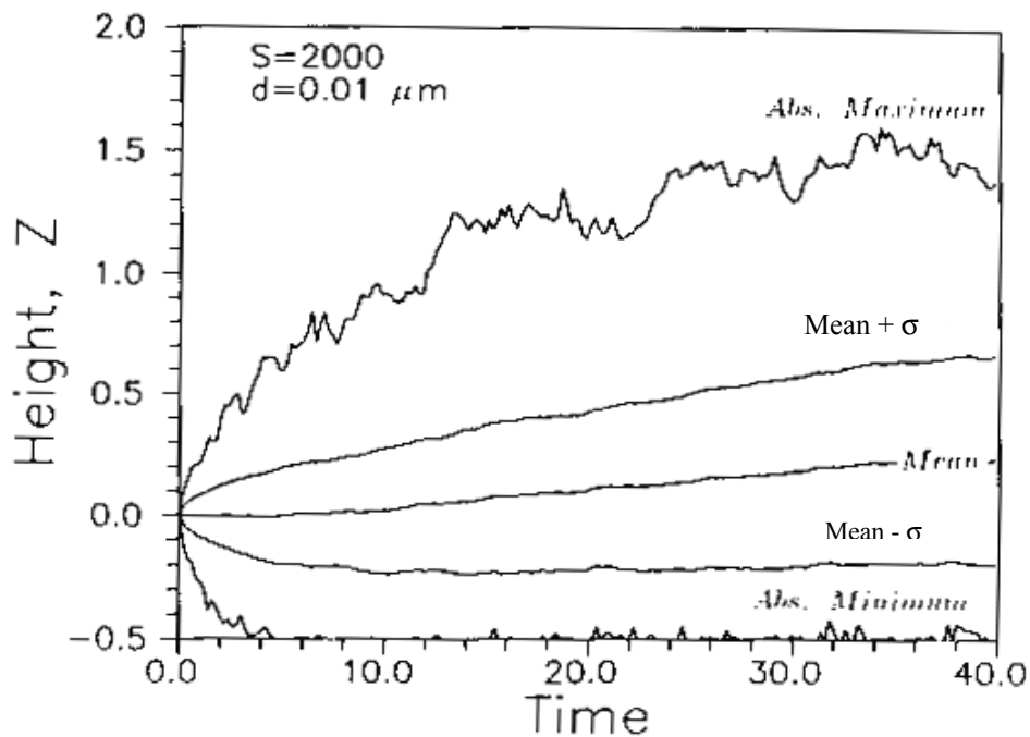
Figure 7. Simulated trajectory statistics for 0.01 μm particles.
